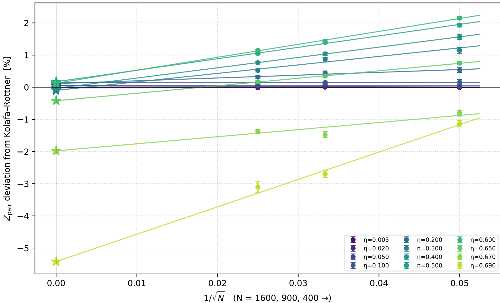
Pair-virial route: finite-size deviation and 1/\sqrt{N} extrapolation (★)
