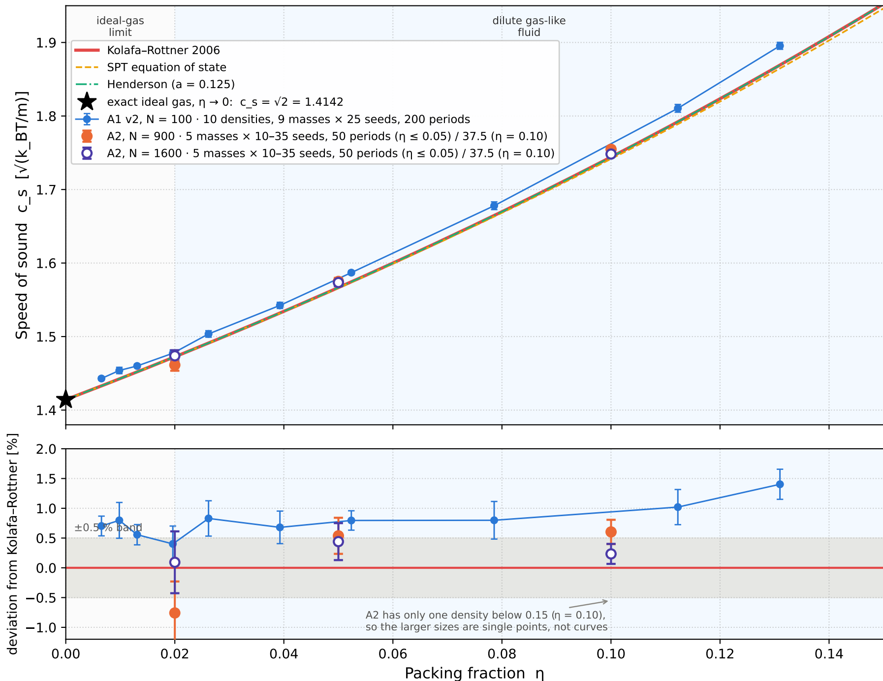
The dilute end: one system size measured densely, two larger sizes at \eta = 0.10 N = 100 (A1 v2) and A2 corrected for box truncation (methods §14)
