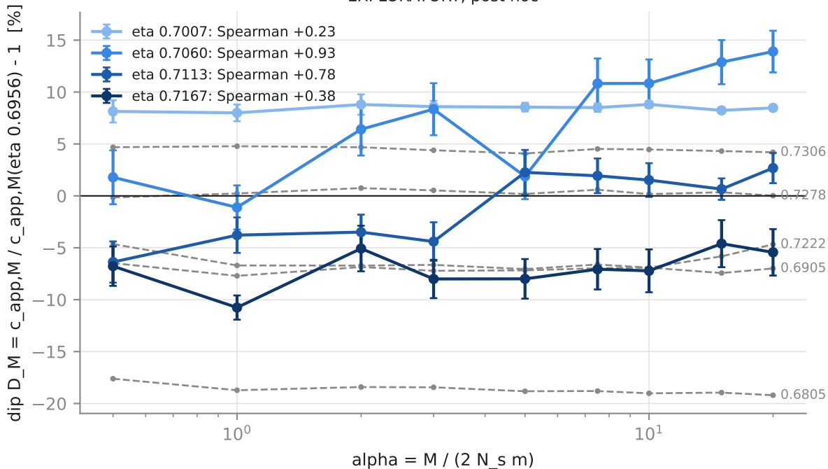
A1v2_20260914: per-mass dip, window cells (blue, light -> dark = rising eta); grey dashed = outside EXPLORATORY, post hoc
