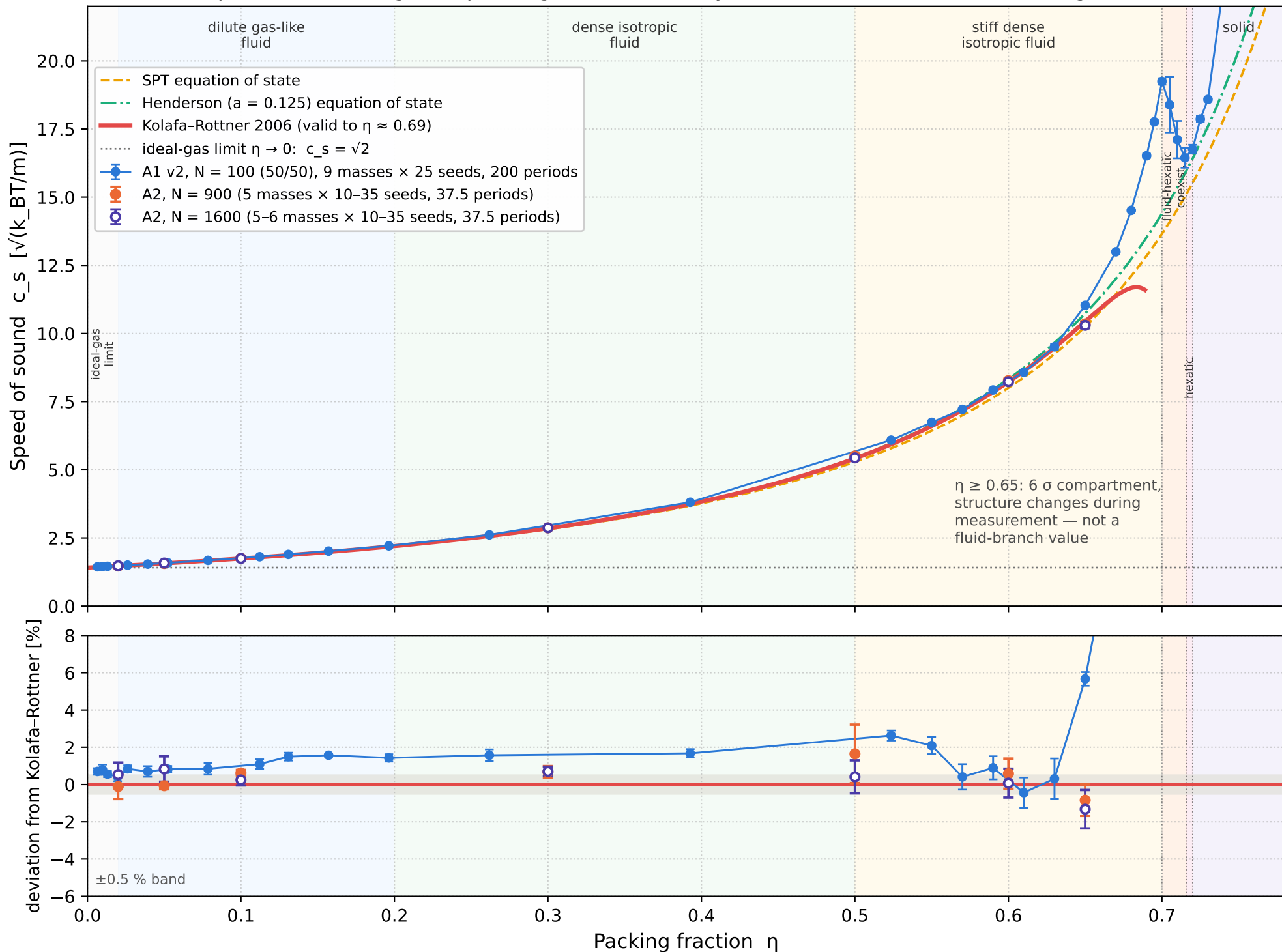
Speed of sound against packing fraction: one system size (N = 100) and two larger ones
