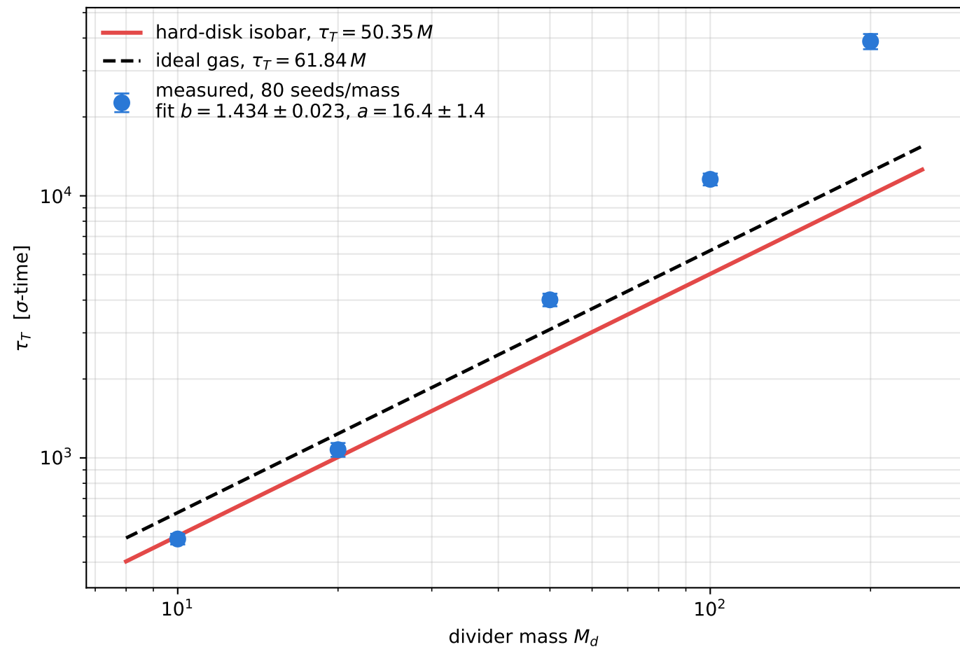
Level 4 mass ladder: \tau_T(M) against the two isobars
