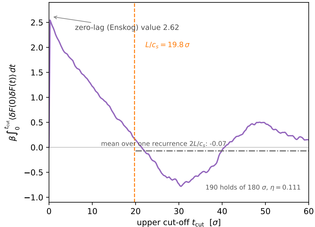
The friction integral cancels at the sound traversal time
