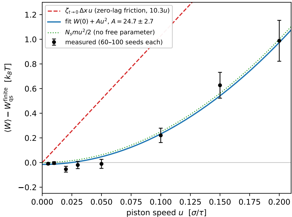
Excess work is second order in the piston speed
