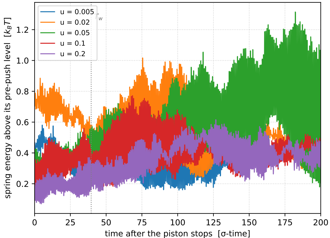
Spring ring-down, seed-averaged
