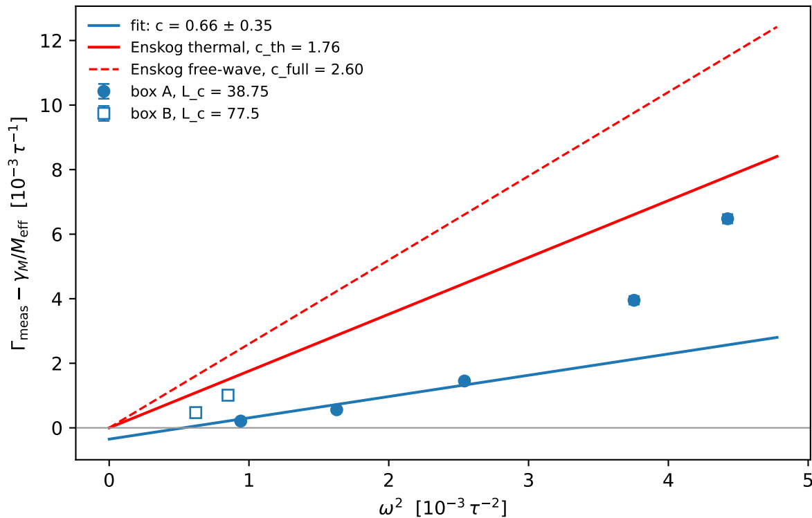
Divider-mode linewidth beyond Mansour friction (261006 ladder, v1)
