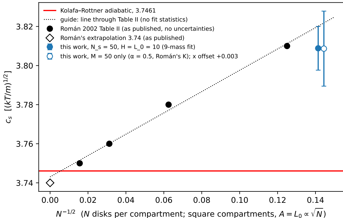
Size series at \eta = \pi/8 : Román 2002 Table II vs Kolafa-Rottner
