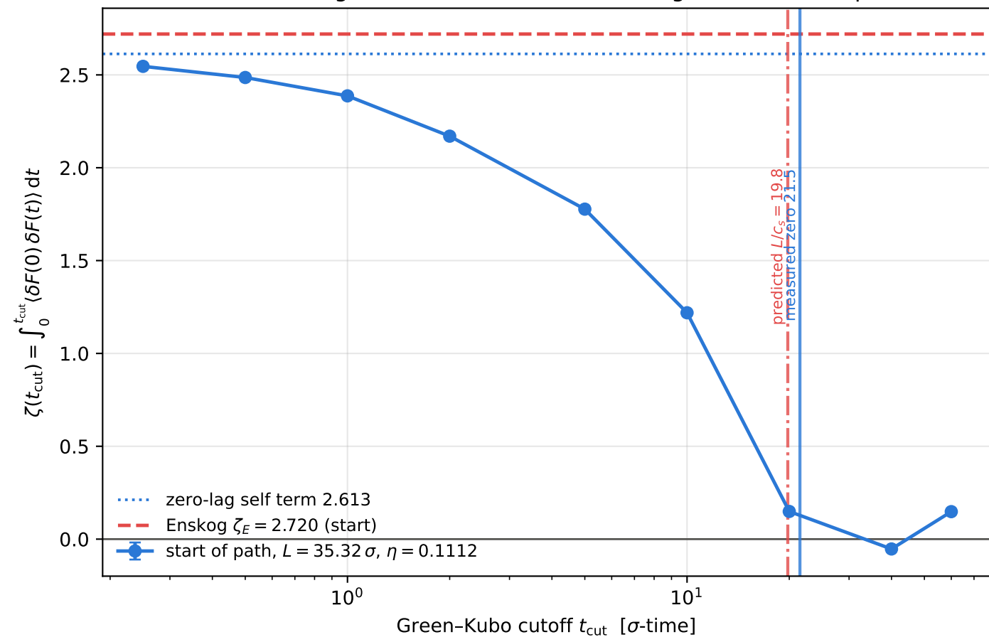
The friction integral dies at the sound-crossing time, not at a plateau
