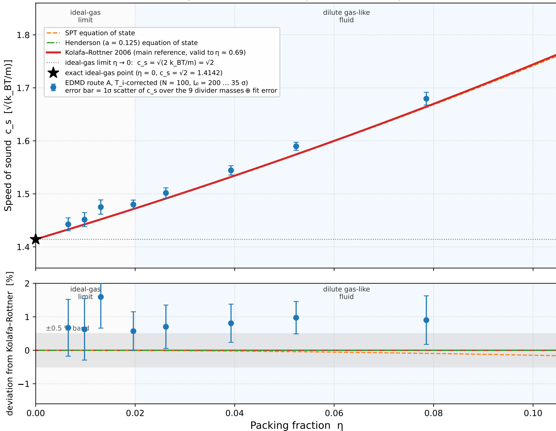
Ideal-gas end of the sound-speed validation ( \eta \leq 0.1 )
