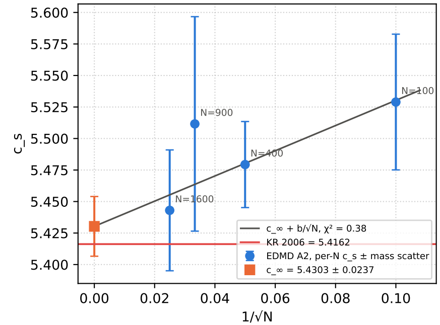
\eta = 0.50 (+0.26 % vs KR, +0.6 \sigma )
