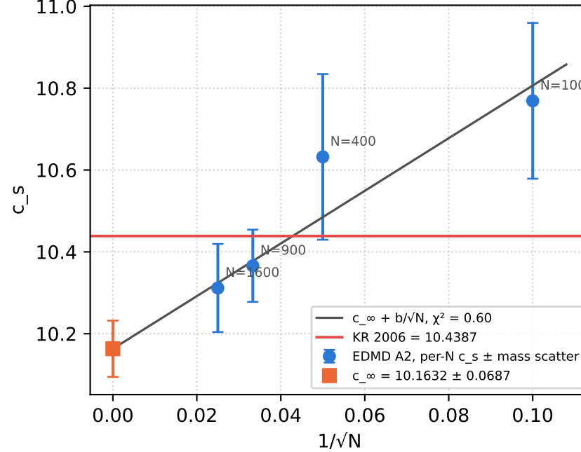
\eta = 0.65 (-2.64 % vs KR, -4.0 \sigma )
