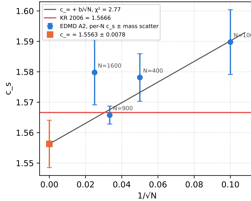
A2, fixed \eta , N ladder: largest FFT bin at f \geq v_{\text{pred}}/2.5 , mean over seeds, through-origin fit over masses
