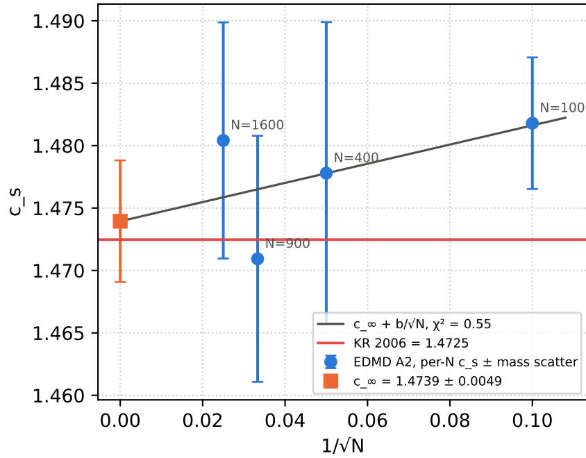
A2, fixed \eta , N ladder: largest FFT bin at f \geq v_{\text{pred}}/2.5 , mean over seeds, through-origin fit over masses
