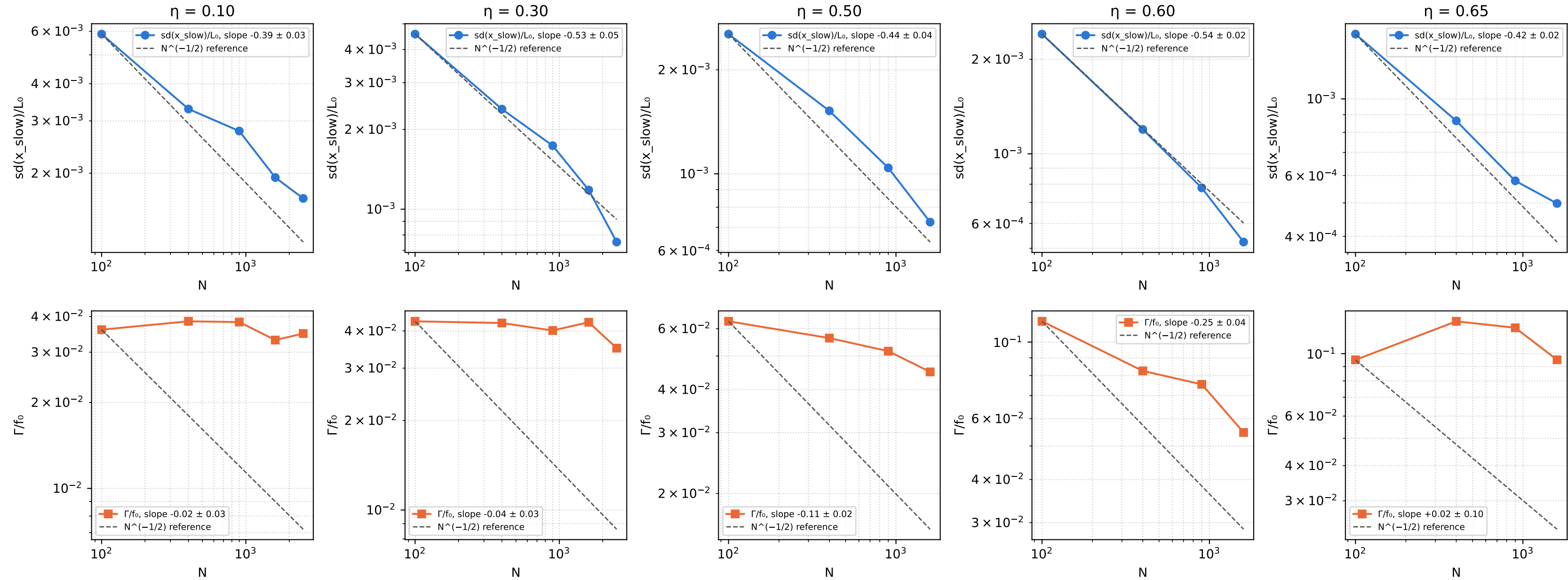
A2: slow-mode amplitude and resonance width against system size (5-period running mean; fits on the same traces)
