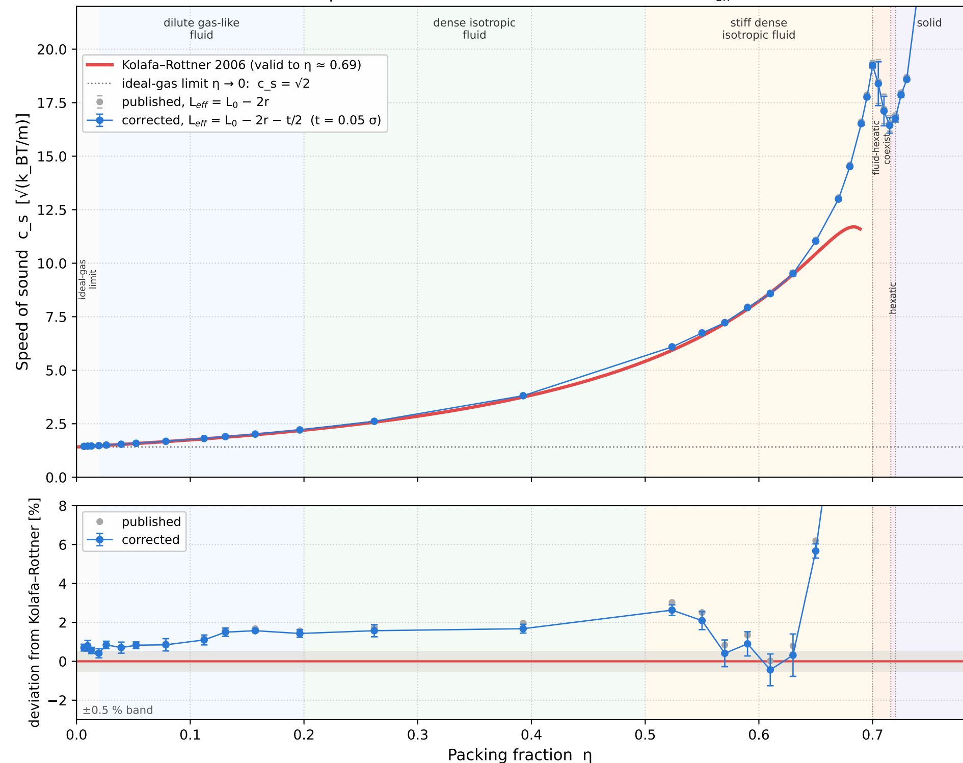
Paper 1 with the divider thickness carried into L_{eff}
