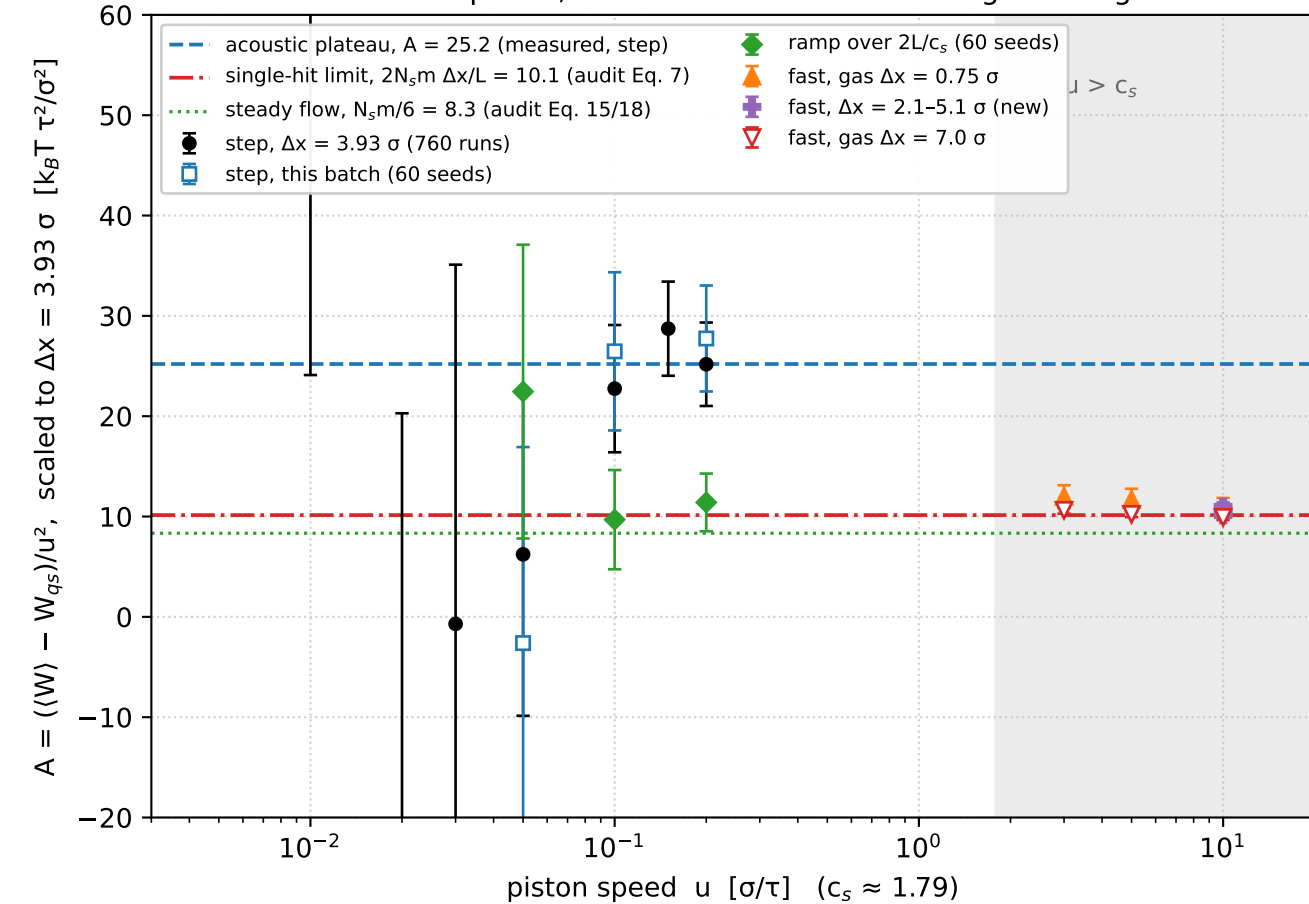
Excess work per u^2 , from the acoustic to the single-hit regime
