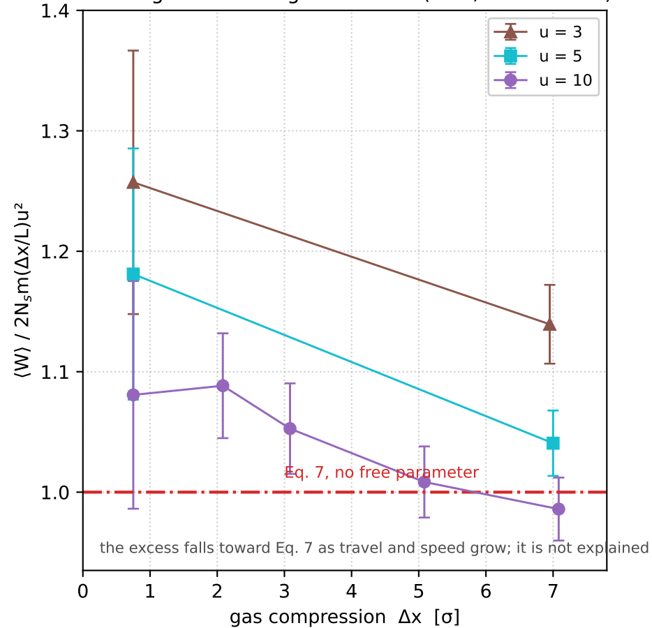
The single-hit limit against travel (new, 2026-09-18)
