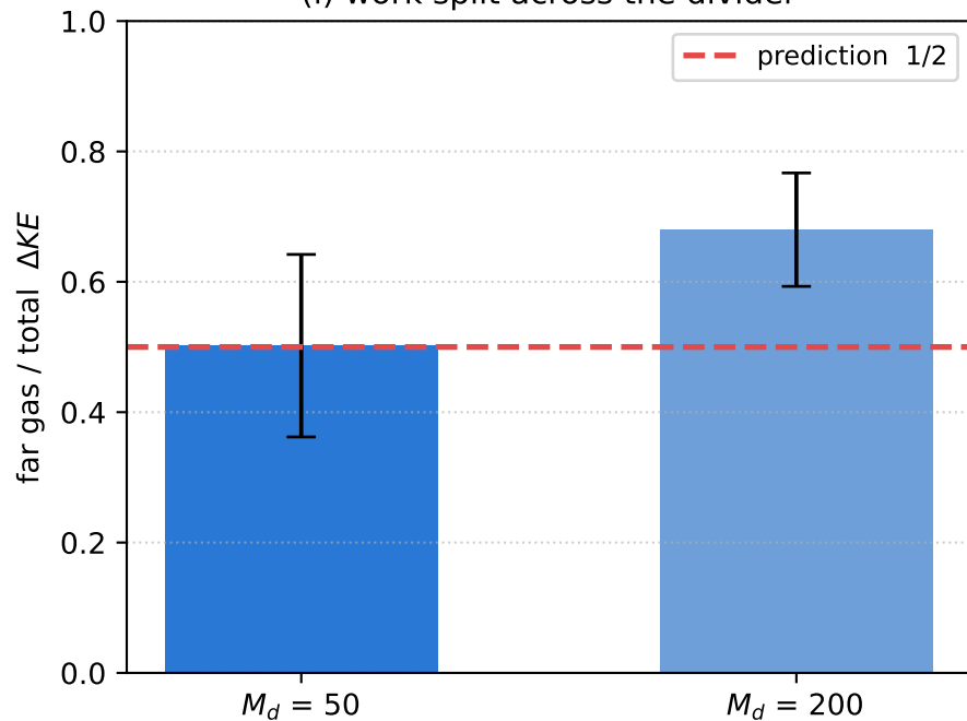
(i) work split across the divider
