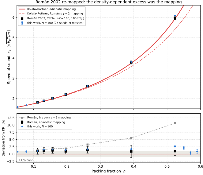
Fig. 5. Román et al. re-mapped. Solid red, Kolafa–Rottner through (1); dashed red, the same equation of state through their \gamma = 2 mapping; black squares, their Table I with their error bars; blue, this work at N = 100 . Lower panel: deviation from Kolafa–Rottner.
