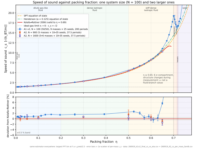
Fig. 4. N = 100 against N = 900 and 1600 at the same densities.
