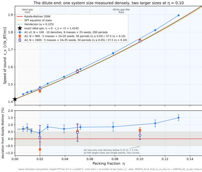
Fig. 3. The dilute end. The N = 100 curve sits 0.5–1.5% above the equation of state; larger systems agree with it within their errors.
