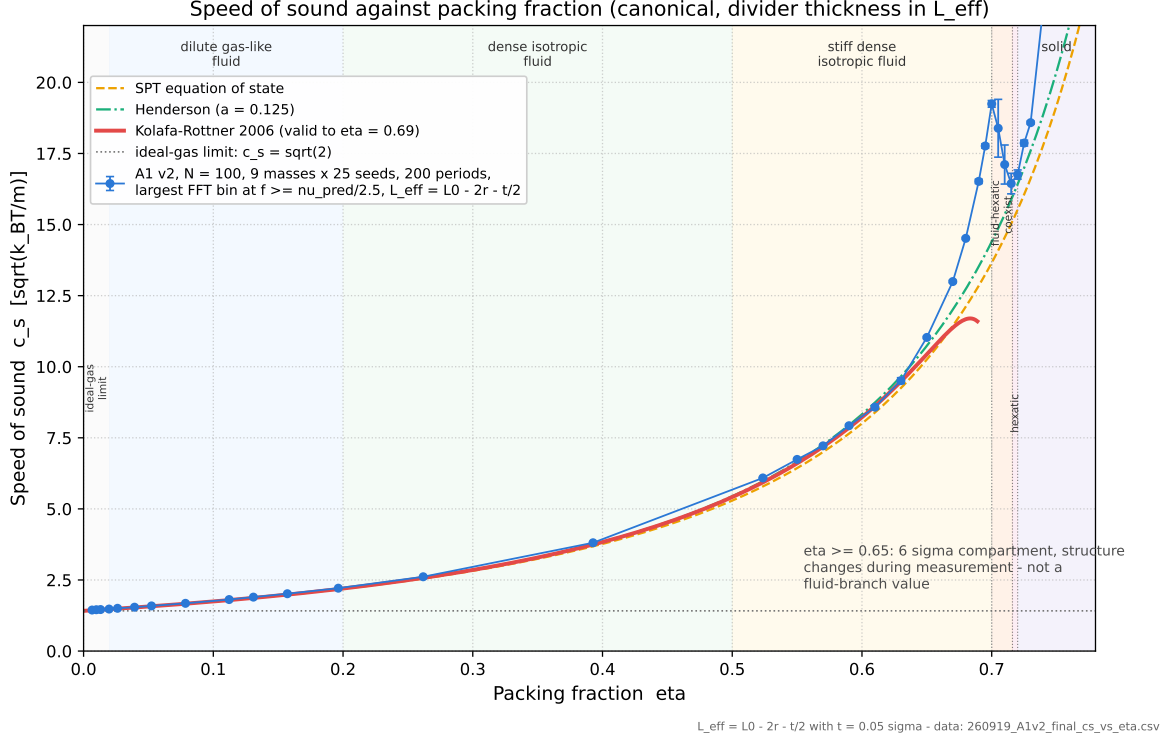
Fig. 2. c_s(\eta) at N = 100 against three equations of state, through (1) with no fitted parameter. Shading marks the approximate regimes. Points beyond \eta \approx 0.69 lie in the coexistence and ordering region where no fluid reference exists; they are shown but are not counted as a deviation from Kolafa–Rottner.
