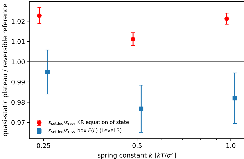
Over-pressure test (points offset in k for legibility)
