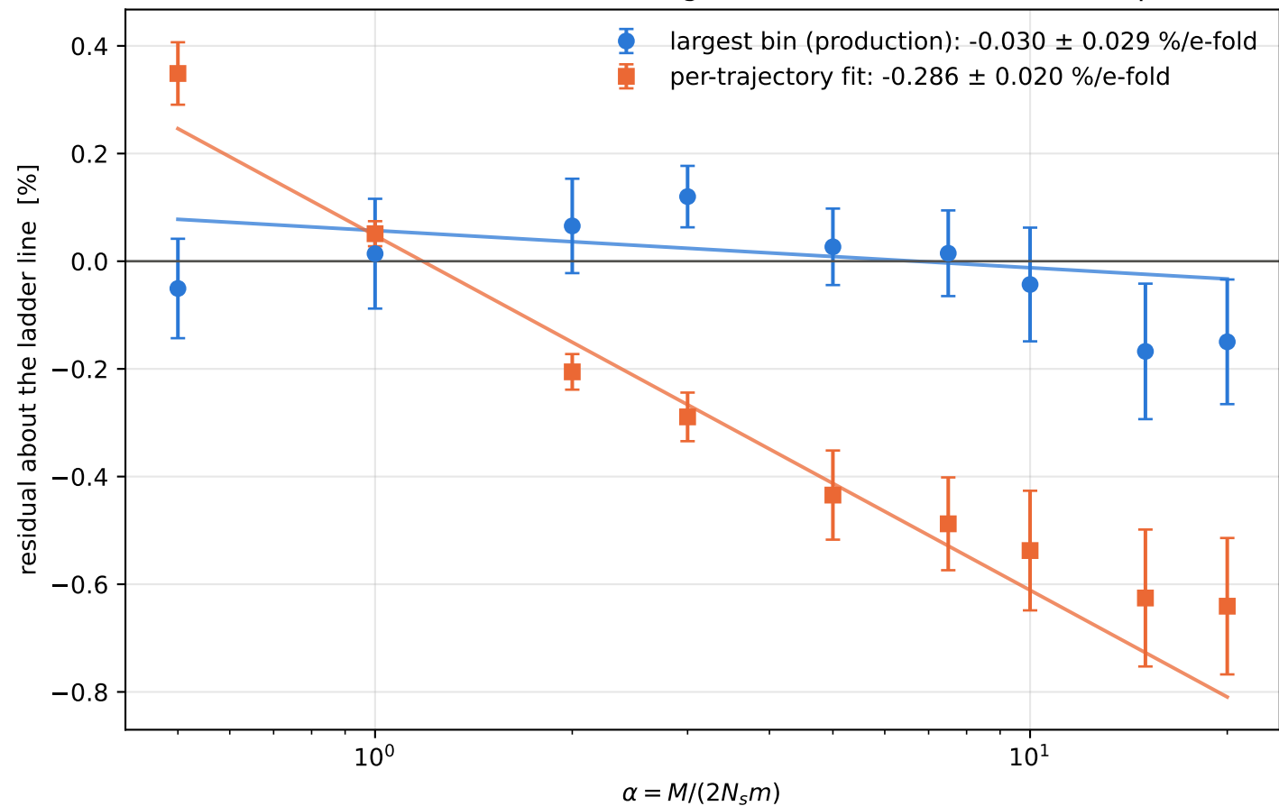
Mass-ladder residual flatness: the largest-bin estimator is mass-independent
