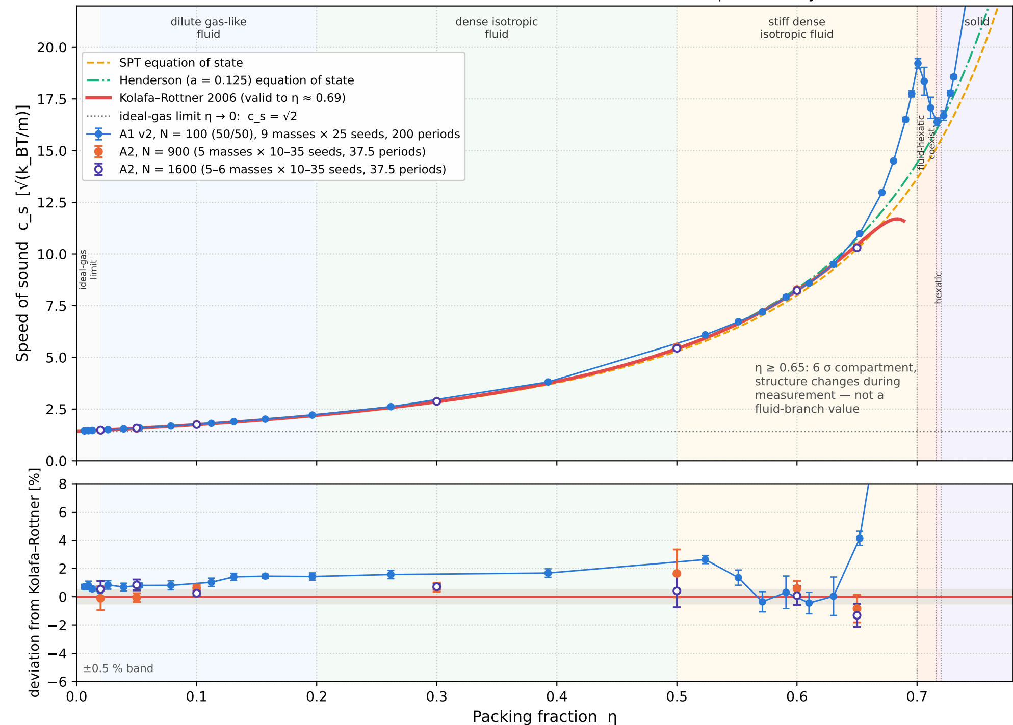
Speed of sound against packing fraction: one system size ( N = 100 ) and two larger ones N = 100 (A1 v2) corrected for box truncation (methods §14); A2 points not yet corrected
