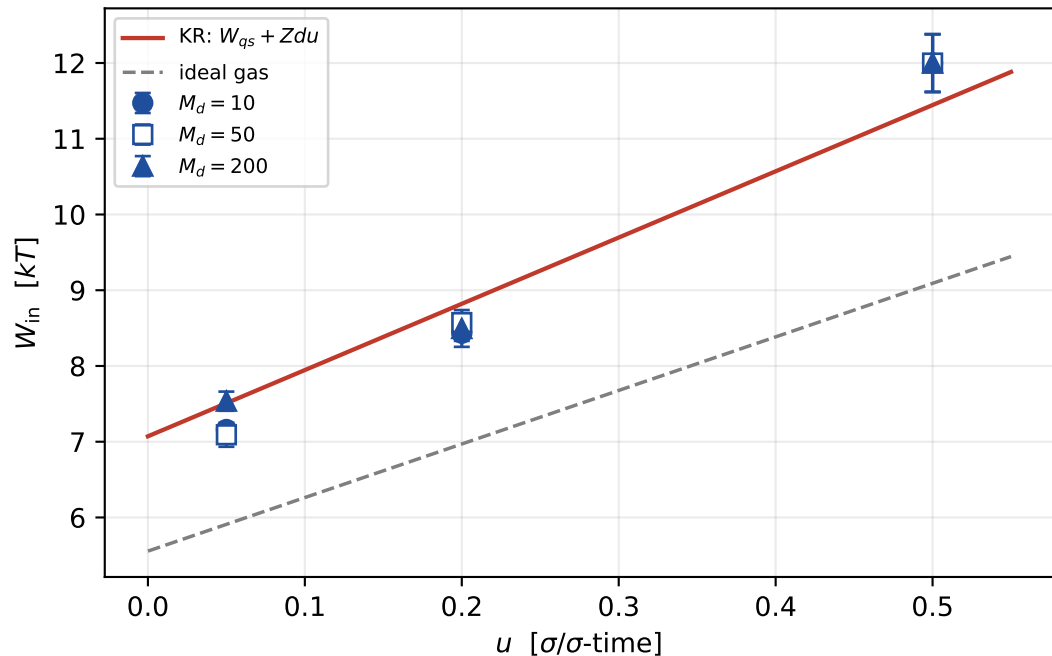
(b) the piston-work ledger
