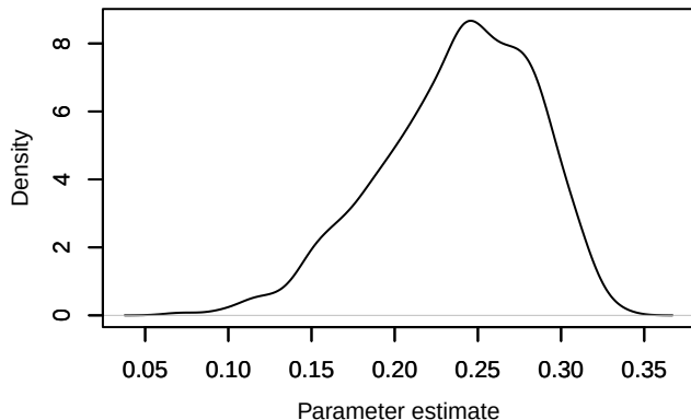
Density – mean_l
