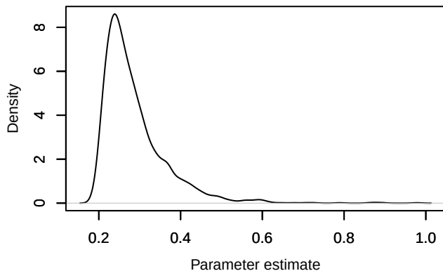
Density – mean_l
