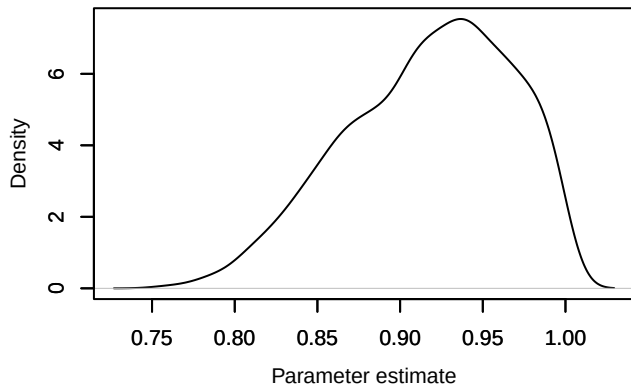
Density – mean_h
