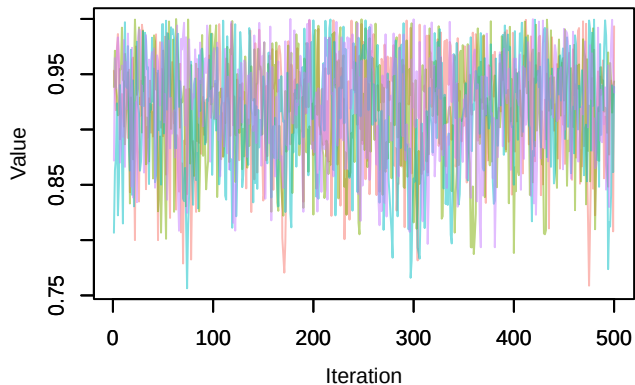
Trace – mean_h
