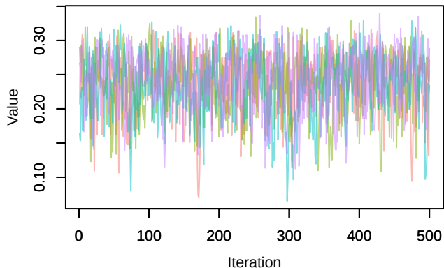
Trace – mean_l
