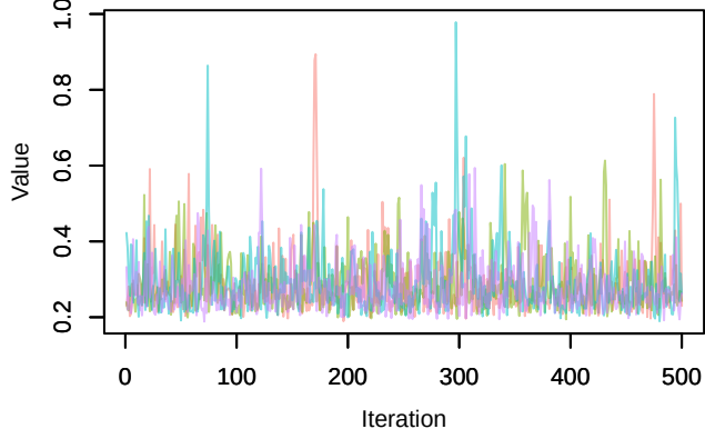
Trace – mean_l
