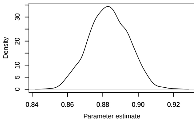
Density – mean_h
