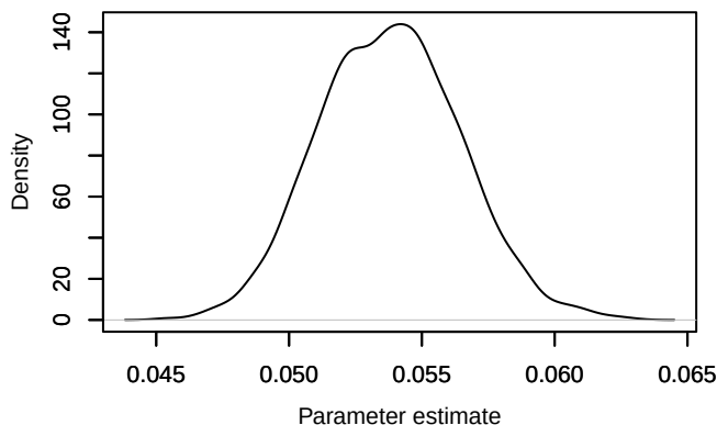
Density – mean_l
