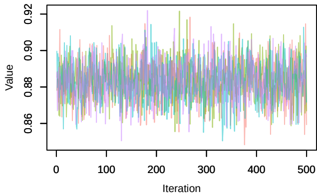
Trace – mean_h
