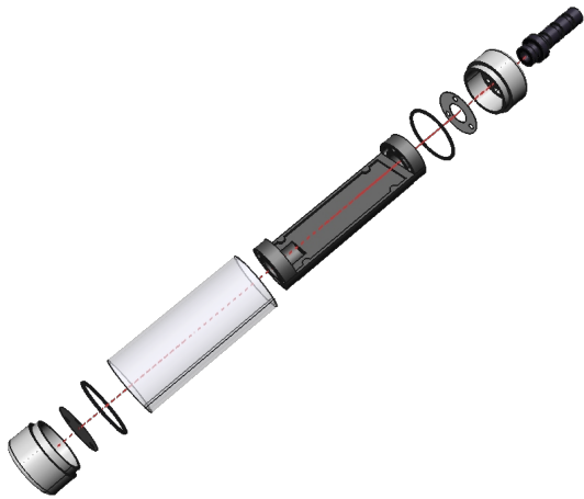
Full Enclosure Exploded View
