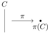
Figure 1.6: A contracted curve
