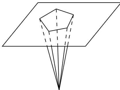
Figure 1.15.: Representing cones
