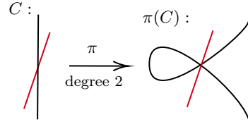
Figure 1.7.: 2nd case
