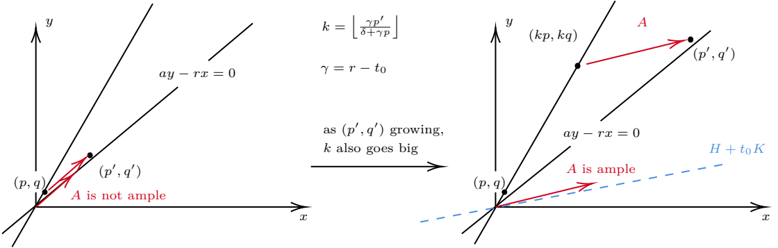
Figure 6.1.: By suitable choice of the parameters, as p' growing the corresponding divisor A are tend to an ample divisor, hence A itself will become ample.
