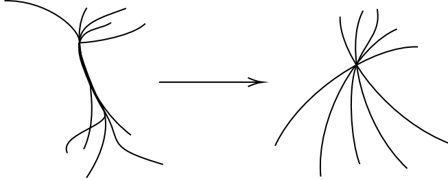
Figure 2.10.: As m growing, the moving part separates from the fixed component.
