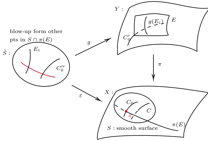
Figure 2.6.: Construction of a rational curve g(E_i) in the E .
