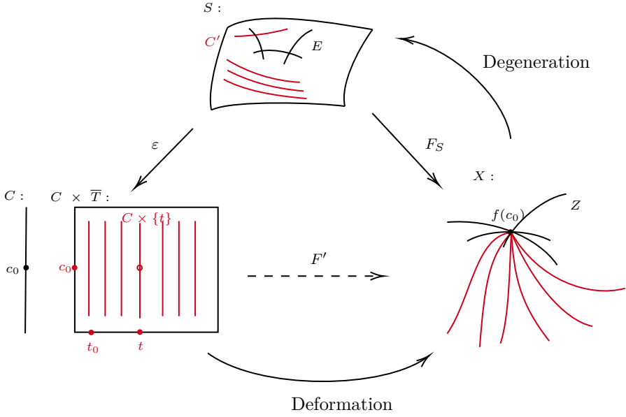
Figure 2.7.: Bend and Break I
