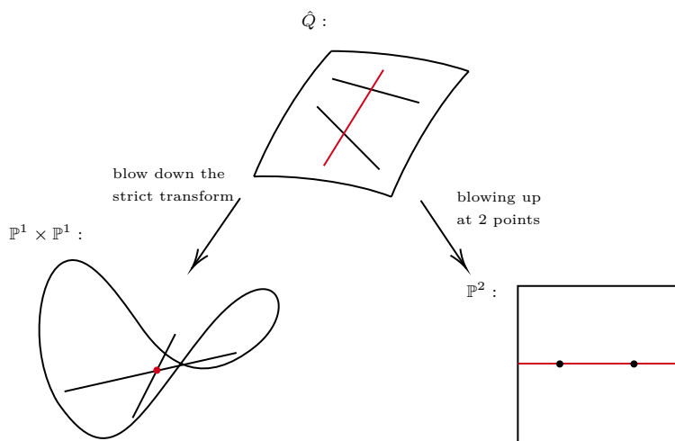
Figure 2.1.: Two distinct minimal surfaces.
