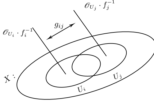
Figure 1.1.: Line Bundle
