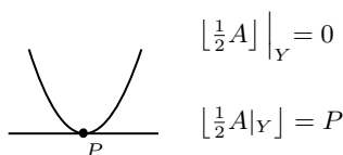
Figure 4.4.: Rounding does not commute with restriction.
