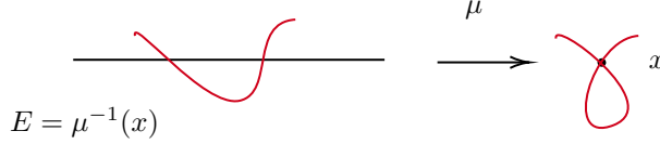
Figure 1.13.: strict transform
