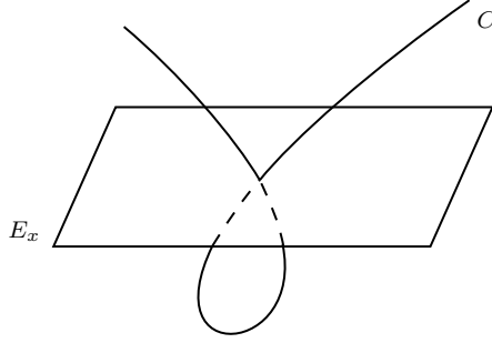
Figure 1.12.: Intersection number bounded below
