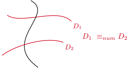
Figure 1.8.: Numerically equivalent
