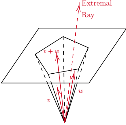
Figure 1.18.: v + w not in extremal ray \mathbf{r} .
