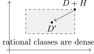
Figure 1.11: Give a small perturbation.
