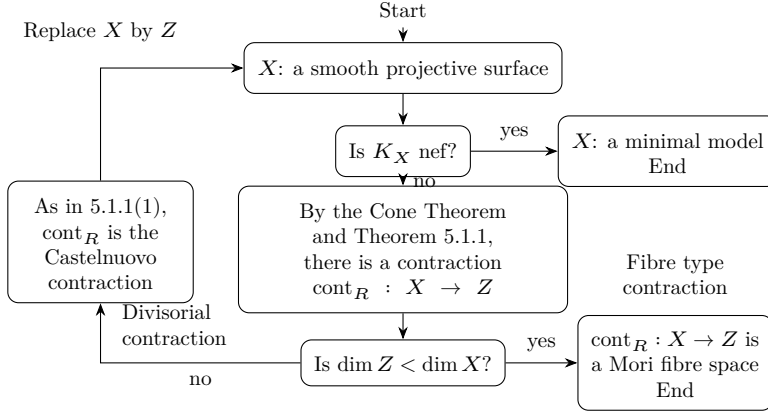
Figure 5.2: Two possibilities correspond to different contractions.
