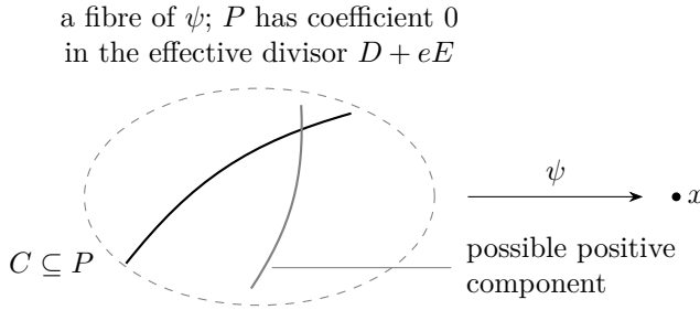
Figure 5.5: A contracted curve C not contained in \text{Supp}(D + eE) . Any intersections with its positive components have non-negative degree.
