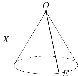
Figure 1.10: The normal quadric cone in \mathbb{P}^3
