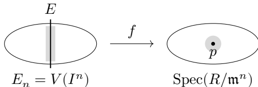
Figure 1.20: The two systems of infinitesimal neighbourhoods have cofinal ideals.
