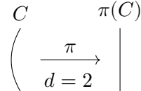
Figure 1.7: A map of degree two
