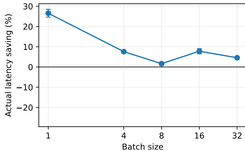
12-thread CPU / CIFAR-10
