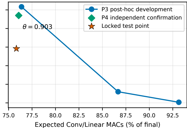
CIFAR-100
