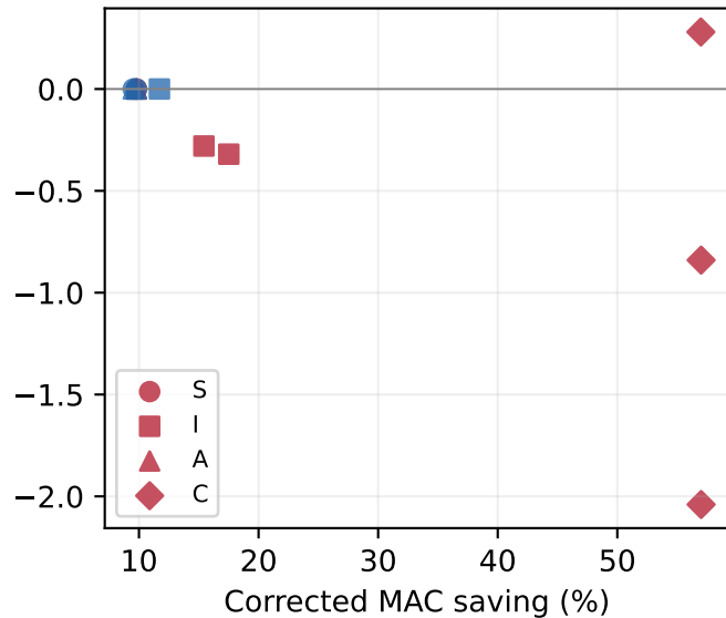
cifar100 / strict
