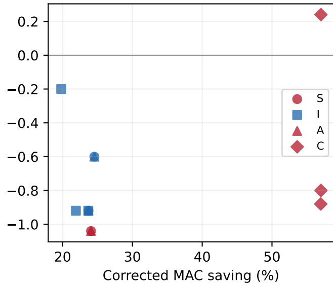
cifar100 / relaxed
