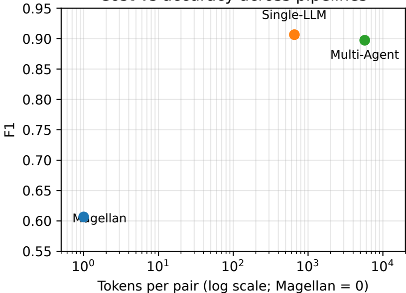
Cost vs accuracy across pipelines
