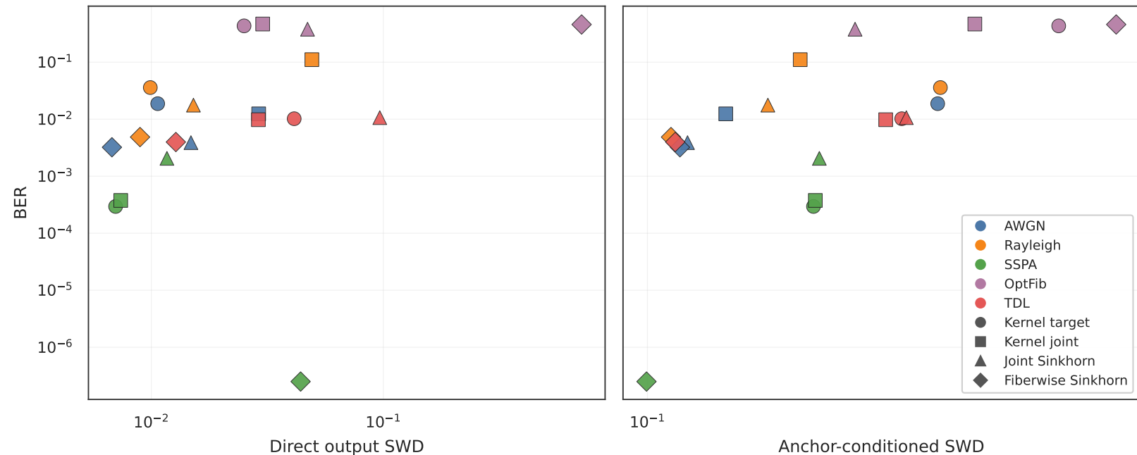
Generator metrics do not fully predict symbolic BER
