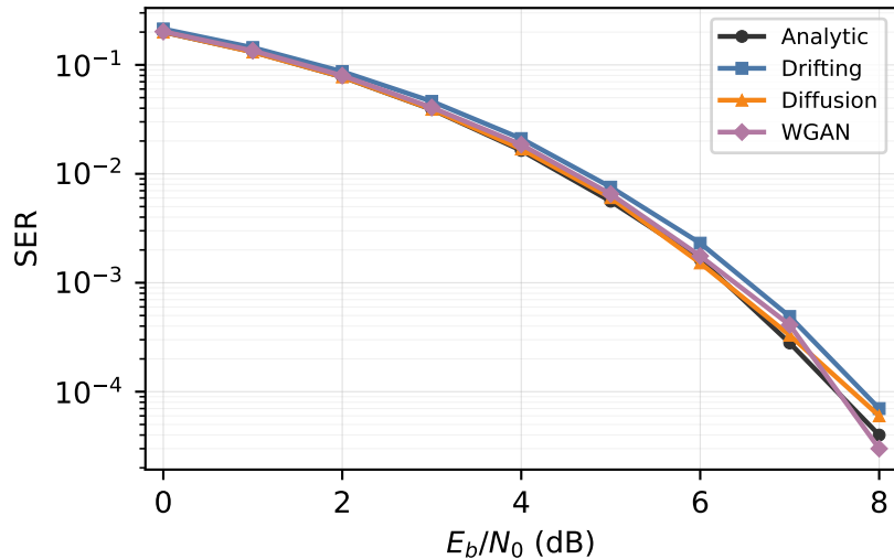
Symbol error rate
