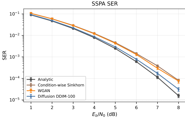
Fig. 6. SSPA SER curve. Symbolic autoencoders are trained through analytic, condition-wise Sinkhorn, WGAN, or DDIM-100 channel implants and evaluated on the analytic channel. Points show seed means with standard-error bars.
