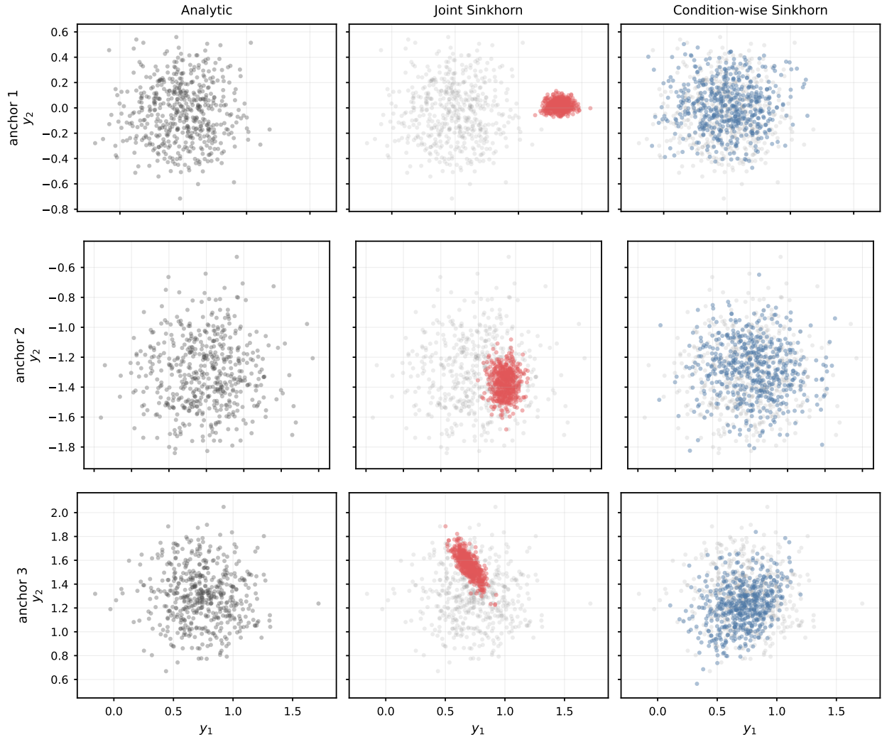
Fig. 3. Fixed-condition SSPA output fibers. Each row fixes one transmitted-symbol anchor x_i and plots repeated channel outputs in the first I/Q plane. The analytic channel is shown in gray. The learned columns overlay generated samples from joint Sinkhorn and condition-wise Sinkhorn on the same analytic cloud. Joint transport can match aspects of the global output distribution while displacing the fixed- x fiber. Condition-wise Sinkhorn better preserves the conditional output law.
