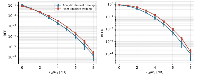
Fig. 8. Long-block TurboAE AWGN check. CNN TurboAE models are trained at block length 64, rate 1/2, and E_b/N_0 = 4 dB, either through the analytic AWGN channel or through the condition-wise Sinkhorn AWGN surrogate. Curves are evaluated on the analytic AWGN channel over 30 seeds. The surrogate preserves the qualitative waterfall trend but remains above the analytic-channel training curve.
