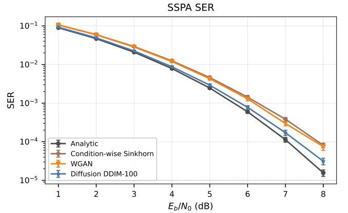
Fig. 5. SSPA SER curve. Symbolic autoencoders are trained through analytic, condition-wise Sinkhorn, WGAN, or DDIM-100 channel implants and evaluated on the analytic channel. Points show seed means with standard-error bars.
