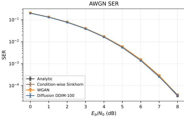
Fig. 3. AWGN SER curve. Symbolic autoencoders are trained through analytic, condition-wise Sinkhorn, WGAN, or DDIM-100 channel implants and evaluated on the analytic channel. Points show seed means with standard-error bars.
