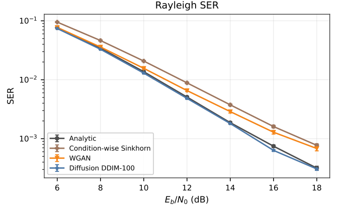
Fig. 4. Rayleigh SER curve. Symbolic autoencoders are trained through analytic, condition-wise Sinkhorn, WGAN, or DDIM-100 channel implants and evaluated on the analytic channel. Points show seed means with standard-error bars.
