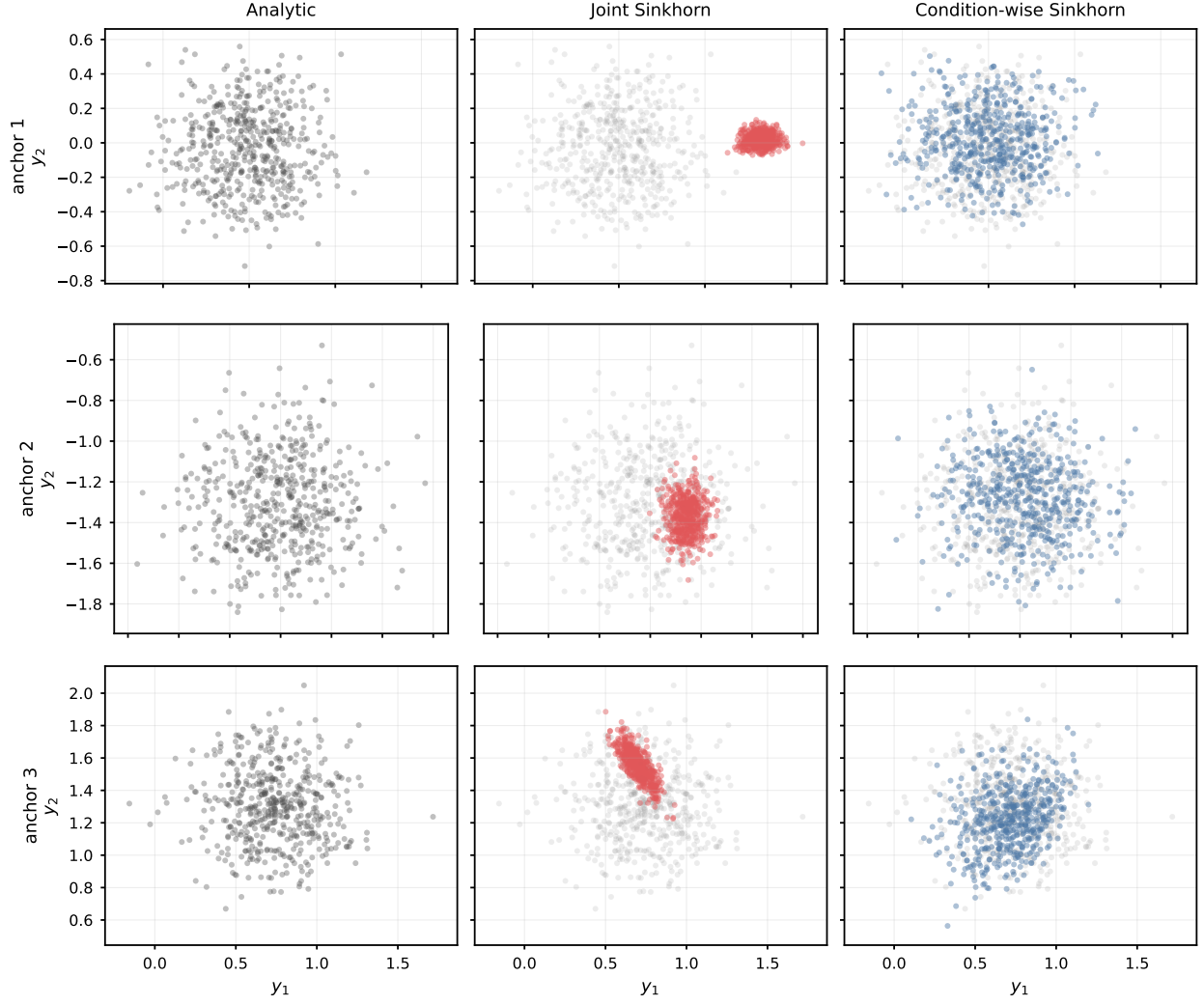
Fig. 1. Fixed-condition SSPA output fibers. Each row fixes one transmitted-symbol anchor x_i and plots repeated channel outputs in the first I/Q plane. The analytic channel is shown in gray. The learned columns overlay generated samples from joint Sinkhorn and condition-wise Sinkhorn on the same analytic cloud. Joint transport can match aspects of the global output distribution while displacing the fixed- x fiber. Condition-wise Sinkhorn better preserves the conditional output law.
