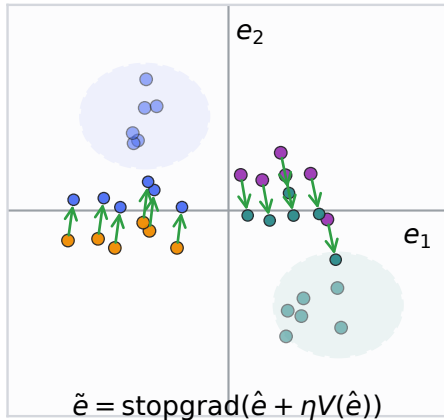
(b) One Drift Update
