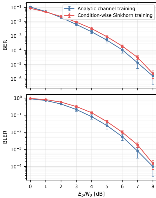
Fig. 3. Long-block TurboAE AWGN check. CNN TurboAE models at block length 64, rate 1/2, are trained through either analytic AWGN or the condition-wise Sinkhorn AWGN surrogate and evaluated on analytic AWGN over 30 seeds. The surrogate preserves the waterfall trend with a measurable gap to analytic-channel training.
