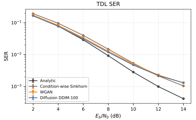
Fig. 7. TDL SER curve. Symbolic autoencoders are trained through analytic, condition-wise Sinkhorn, WGAN, or DDIM-100 channel implants and evaluated on the analytic channel. Points show seed means with standard-error bars.
