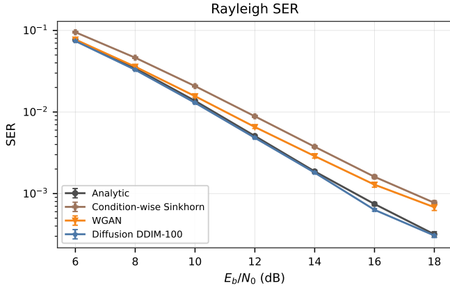
Fig. 5. Rayleigh SER curve. Symbolic autoencoders are trained through analytic, condition-wise Sinkhorn, WGAN, or DDIM-100 channel implants and evaluated on the analytic channel. Points show seed means with standard-error bars.
