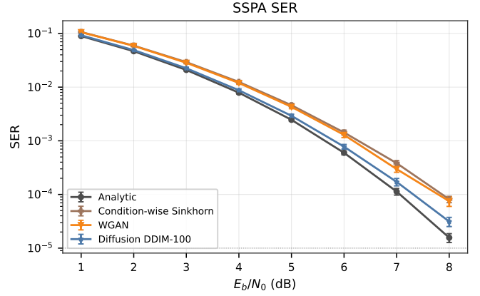
Fig. 6. SSPA SER curve. Symbolic autoencoders are trained through analytic, condition-wise Sinkhorn, WGAN, or DDIM-100 channel implants and evaluated on the analytic channel. Points show seed means with standard-error bars.
