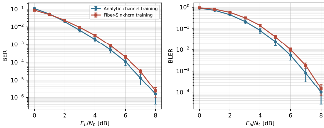
Fig. 8. Long-block TurboAE AWGN check. CNN TurboAE models are trained at block length 64, rate 1/2, and E_b/N_0 = 4 dB, either through the analytic AWGN channel or through the condition-wise Sinkhorn AWGN surrogate. Curves are evaluated on the analytic AWGN channel over 30 seeds. The surrogate preserves the qualitative waterfall trend but remains above the analytic-channel training curve.
