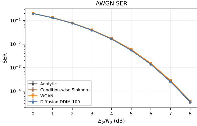
Fig. 4. AWGN SER curve. Symbolic autoencoders are trained through analytic, condition-wise Sinkhorn, WGAN, or DDIM-100 channel implants and evaluated on the analytic channel. Points show seed means with standard-error bars.
