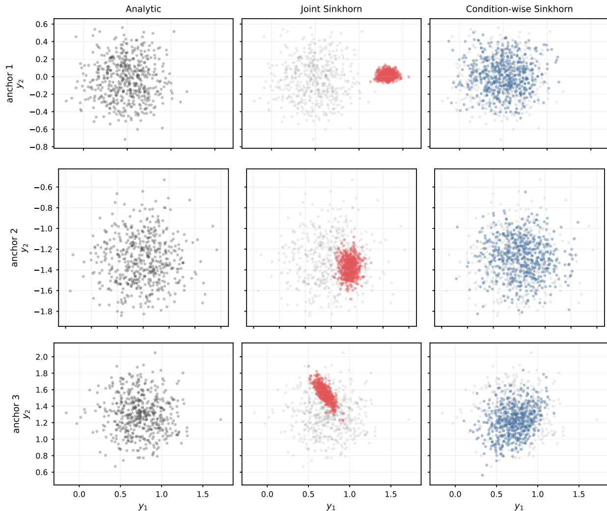
Fig. 3. Fixed-condition SSPA output fibers. Each row fixes one transmitted-symbol anchor x_i and plots repeated channel outputs in the first I/Q plane. The analytic channel is shown in gray. The learned columns overlay generated samples from joint Sinkhorn and condition-wise Sinkhorn on the same analytic cloud. Joint transport can match aspects of the global output distribution while displacing the fixed- x fiber. Condition-wise Sinkhorn better preserves the conditional output law.
