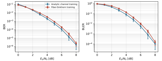
Fig. 9. Long-block TurboAE AWGN check. CNN TurboAE models are trained at block length 64, rate 1/2, and E_b/N_0 = 4 dB, either through the analytic AWGN channel or through the condition-wise Sinkhorn AWGN surrogate. Curves are evaluated on the analytic AWGN channel over 30 seeds. The surrogate preserves the qualitative waterfall trend but remains above the analytic-channel training curve.
