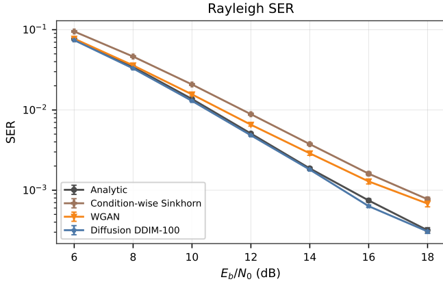
Fig. 6. Rayleigh SER curve. Symbolic autoencoders are trained through analytic, condition-wise Sinkhorn, WGAN, or DDIM-100 channel implants and evaluated on the analytic channel. Points show seed means with standard-error bars.
