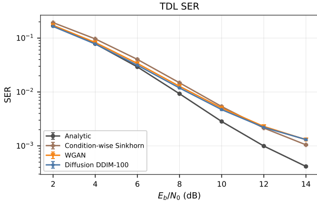
Fig. 8. TDL SER curve. Symbolic autoencoders are trained through analytic, condition-wise Sinkhorn, WGAN, or DDIM-100 channel implants and evaluated on the analytic channel. Points show seed means with standard-error bars.
