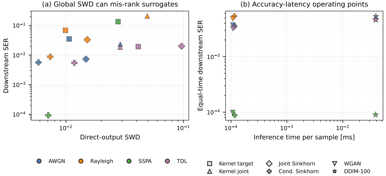
Fig. 4. Metric mismatch and accuracy-latency diagnostics. Panel (a) compares direct-output SWD with downstream symbolic SER for W-Flow ablations. The plotted points use the same aggregate sources as Tables V and VIII. Panel (b) compares learned channel implants by inference latency and equal-wall-clock symbolic SER from Table IX. Colors denote channels and marker shapes denote methods.
