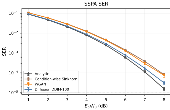
Fig. 7. SSPA SER curve. Symbolic autoencoders are trained through analytic, condition-wise Sinkhorn, WGAN, or DDIM-100 channel implants and evaluated on the analytic channel. Points show seed means with standard-error bars.
