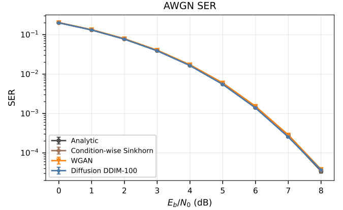
Fig. 5. AWGN SER curve. Symbolic autoencoders are trained through analytic, condition-wise Sinkhorn, WGAN, or DDIM-100 channel implants and evaluated on the analytic channel. Points show seed means with standard-error bars.
