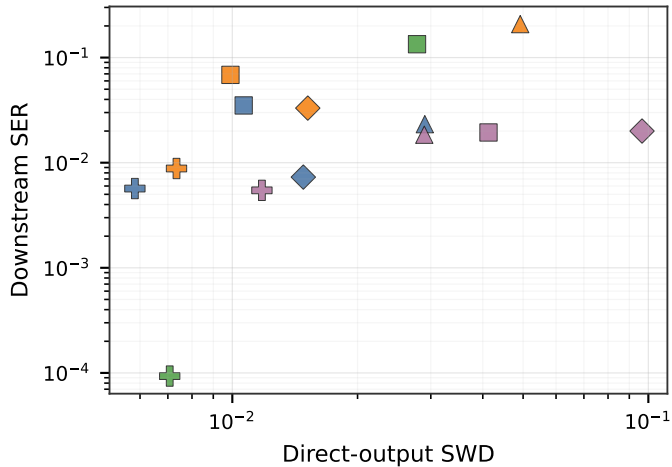
(a) Global SWD can mis-rank surrogates
