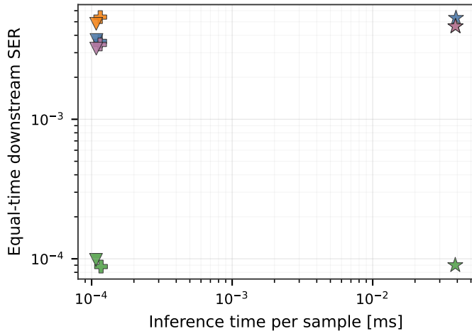
(b) Accuracy-latency operating points
