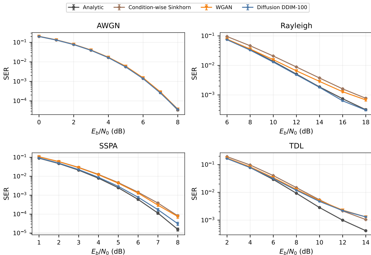
Fig. 2. SER curves for learned channel surrogates. Symbolic autoencoders are trained through each surrogate at the nominal training point and evaluated on the analytic channel over an E_b/N_0 grid for AWGN, Rayleigh, SSPA, and TDL. Curves report seed means with standard-error bars; points below the single-run Monte Carlo resolution are clipped to the dotted reporting floor and marked as upper bounds.
