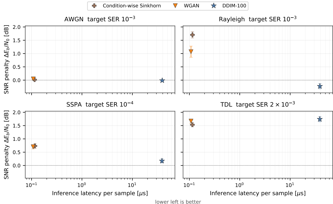
Fig. 3. SNR penalty versus inference latency. Each point reports the additional E_b/N_0 required to reach the target SER shown in the panel title, relative to analytic-channel training on the same channel. Penalties are interpolated seed-wise from the SER curves in Fig. 2 and shown as mean \pm standard error. Latency is the local CUDA inference time per generated channel sample from Table VI. Lower left is better.
