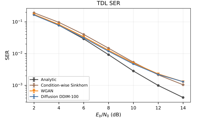
Fig. 6. TDL SER curve. Symbolic autoencoders are trained through analytic, condition-wise Sinkhorn, WGAN, or DDIM-100 channel implants and evaluated on the analytic channel. Points show seed means with standard-error bars.
