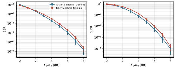
Fig. 7. Long-block TurboAE AWGN check. CNN TurboAE models are trained at block length 64, rate 1/2, and E_b/N_0 = 4 dB, either through the analytic AWGN channel or through the condition-wise Sinkhorn AWGN surrogate. Curves are evaluated on the analytic AWGN channel over 30 seeds. The surrogate preserves the qualitative waterfall trend but remains above the analytic-channel training curve.
