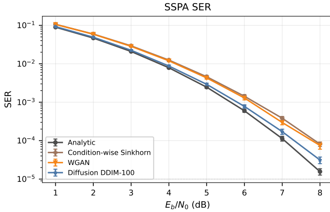
Fig. 5. SSPA SER curve. Symbolic autoencoders are trained through analytic, condition-wise Sinkhorn, WGAN, or DDIM-100 channel implants and evaluated on the analytic channel. Points show seed means with standard-error bars.
