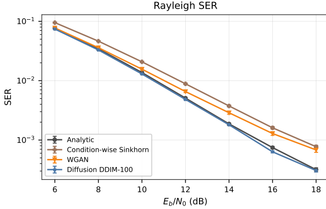
Fig. 4. Rayleigh SER curve. Symbolic autoencoders are trained through analytic, condition-wise Sinkhorn, WGAN, or DDIM-100 channel implants and evaluated on the analytic channel. Points show seed means with standard-error bars.
