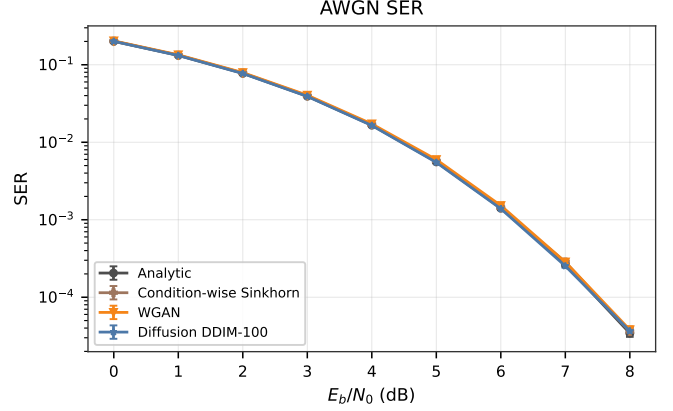
Fig. 3. AWGN SER curve. Symbolic autoencoders are trained through analytic, condition-wise Sinkhorn, WGAN, or DDIM-100 channel implants and evaluated on the analytic channel. Points show seed means with standard-error bars.
