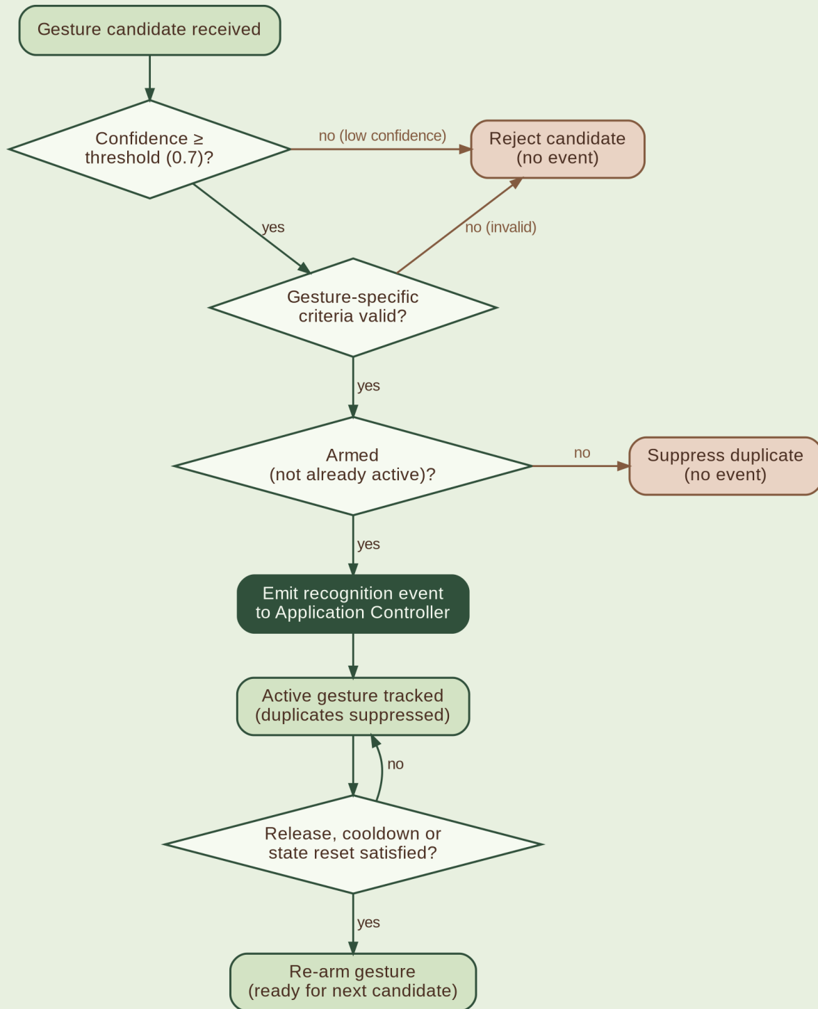
Figure SDP-05: Recognition validation and event re-arming. Rejection and suppression paths are shown in tan.
