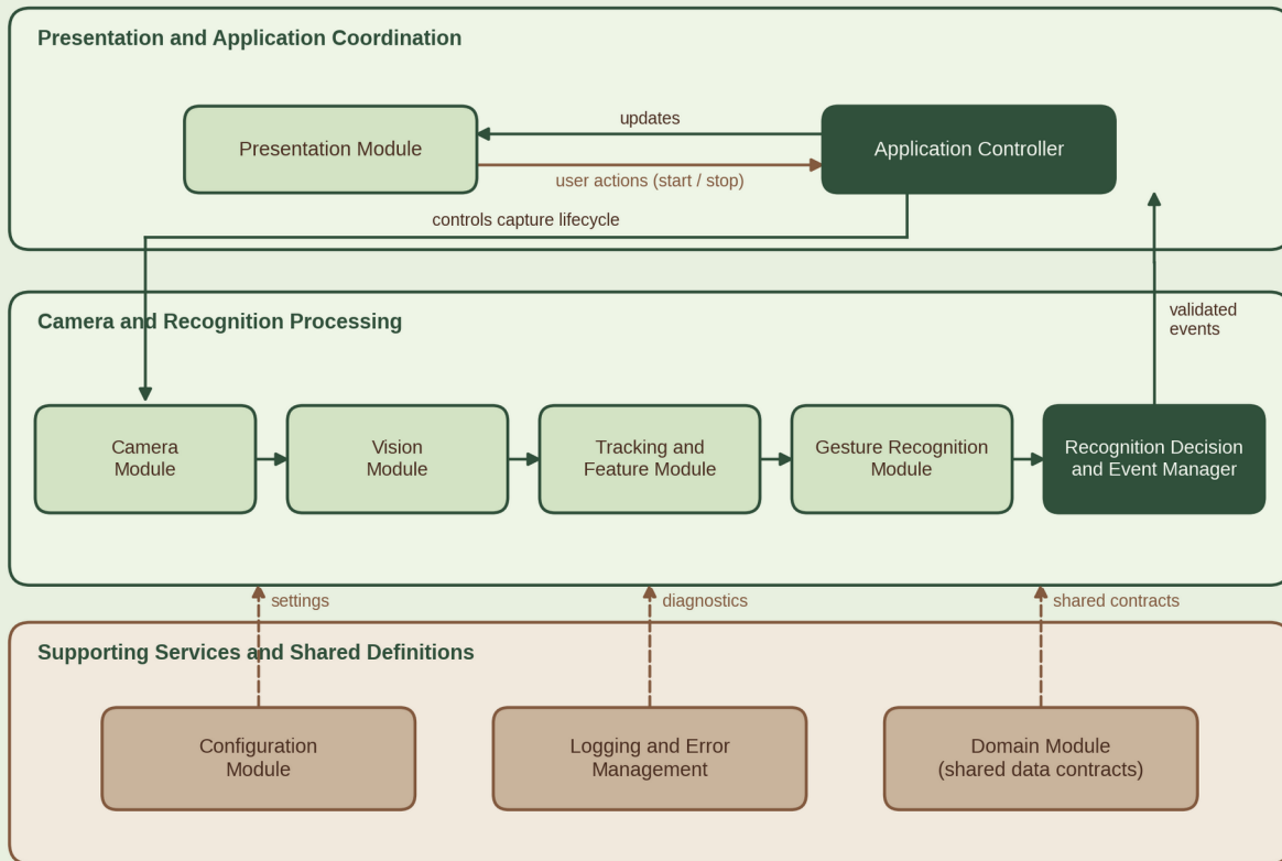
Figure SDP-01: Software module decomposition: ten modules in three logical areas.
