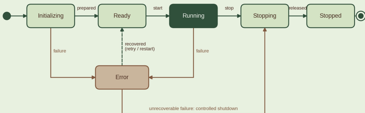
Figure SDP-02: Application lifecycle state machine, including error recovery and controlled shutdown.
