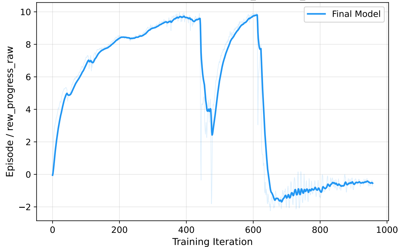
Training Curve: Episode / rew_progress_raw
