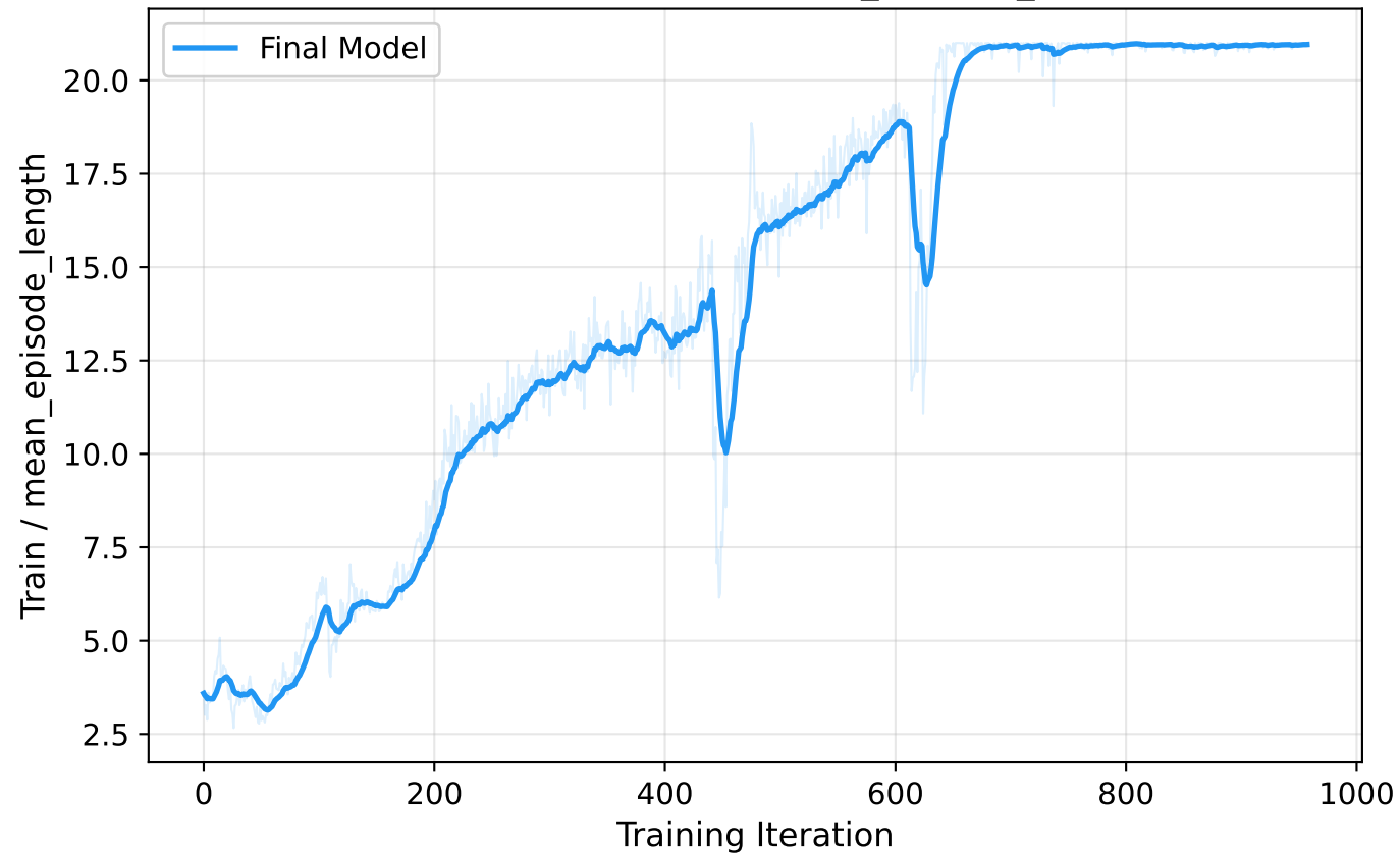
Training Curve: Train / mean_episode_length
