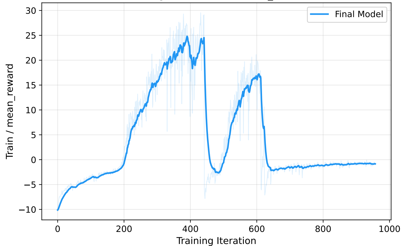
Training Curve: Train / mean_reward
