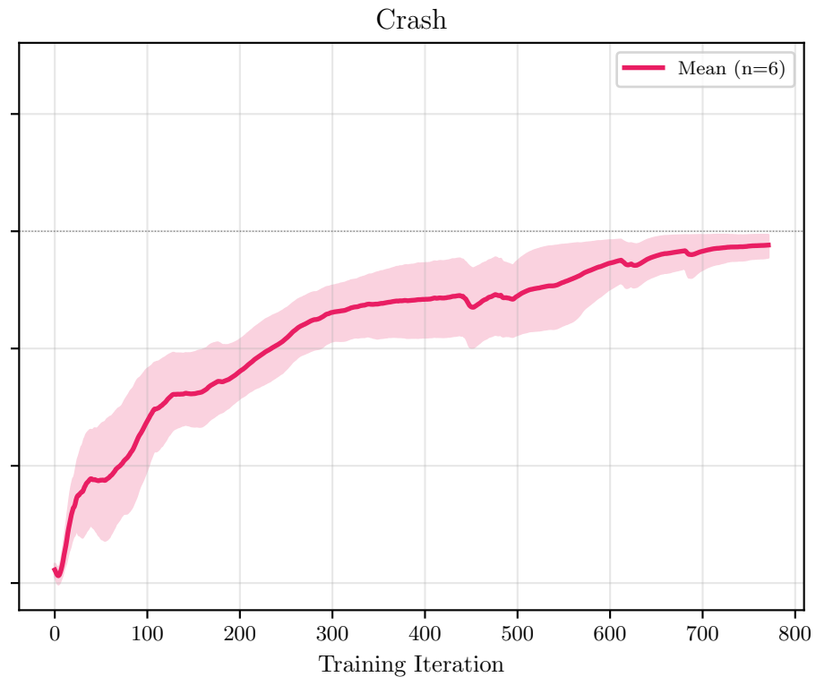
Reward Components: Mean with 95% Bootstrap CI (6 Seeds)
